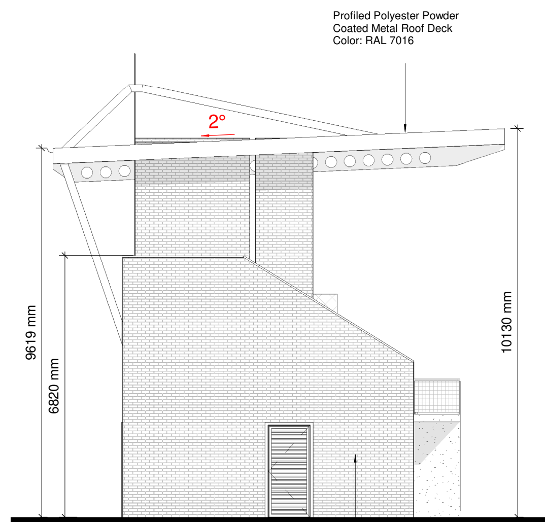
3 Elevation - South 1 : 100
