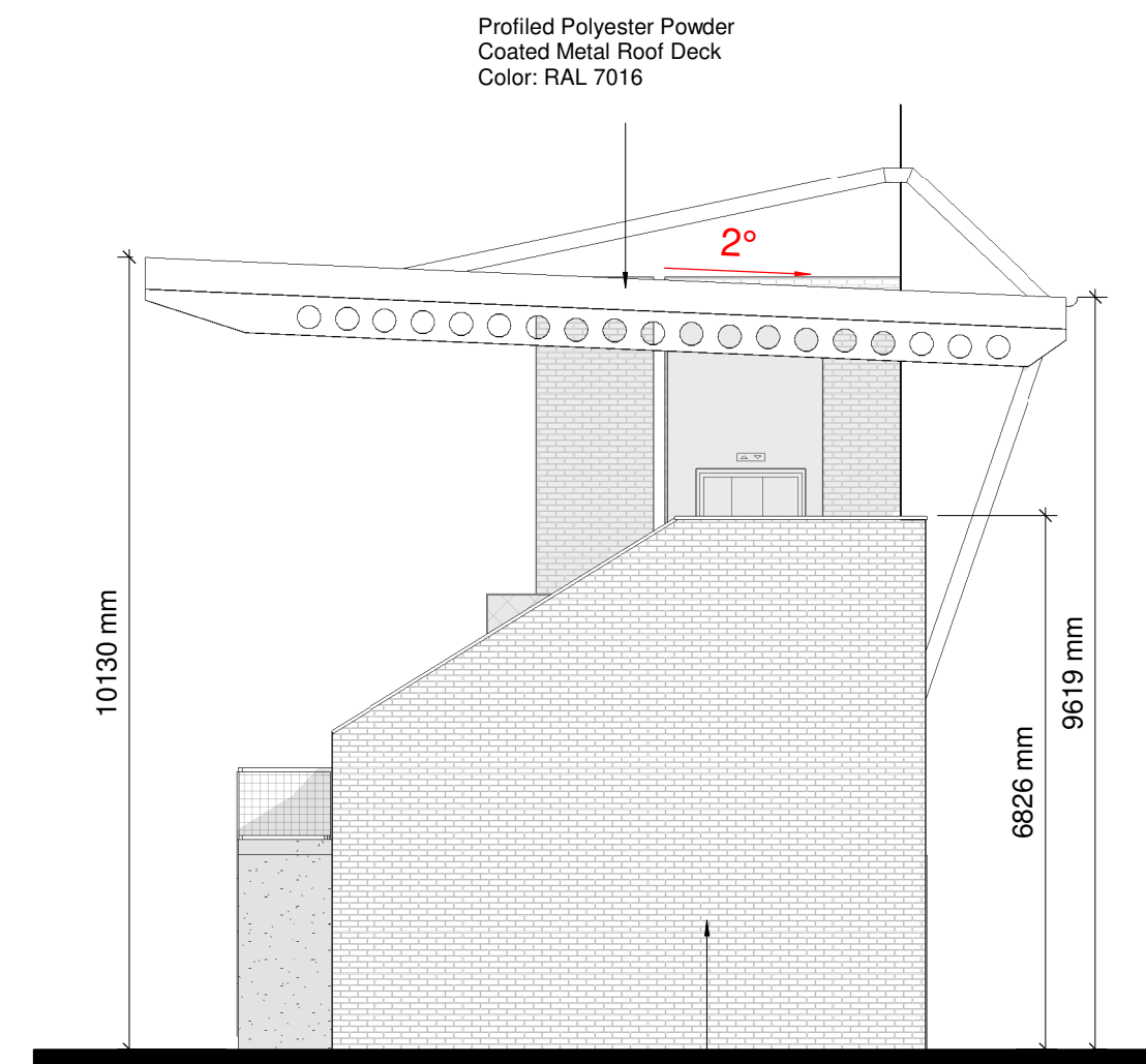
4 Elevation - North 1 : 100
