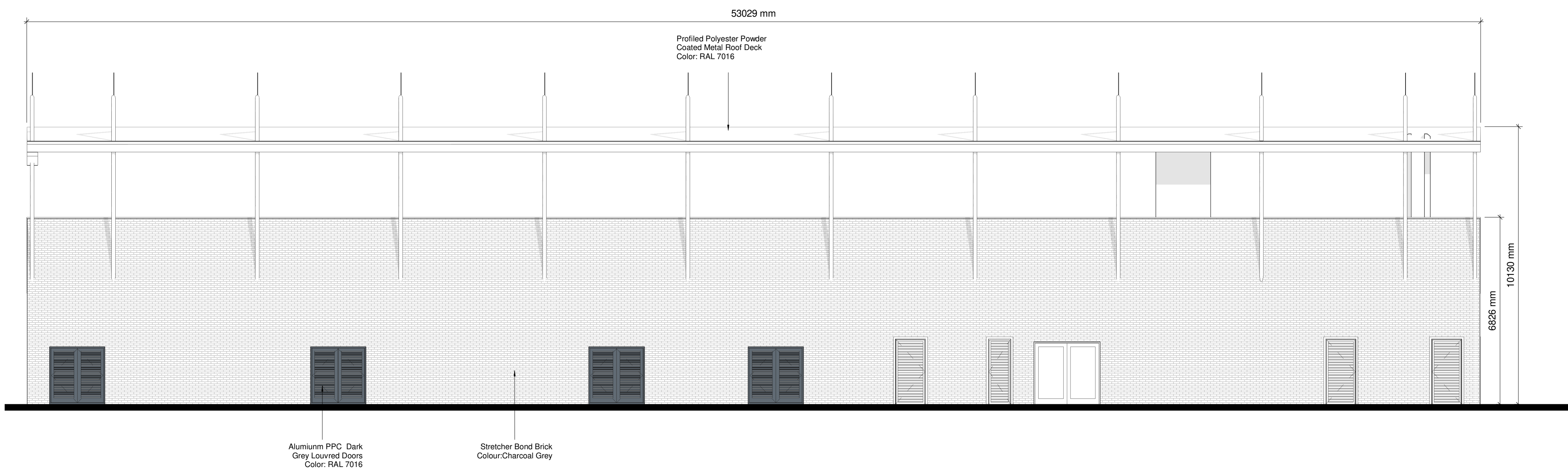
2 Elevation - East 1 : 100
