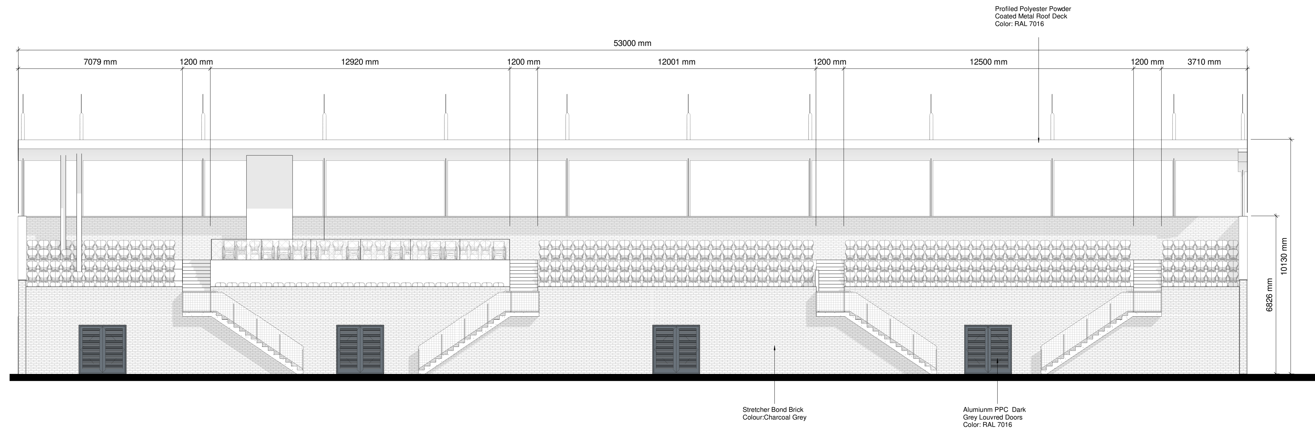
1 Elevation - West 1 : 100
